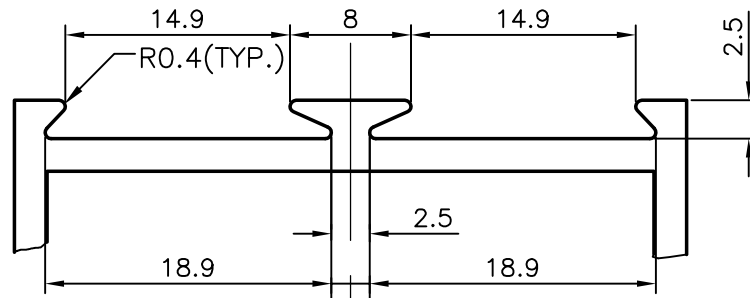
DETAIL AT "X"
