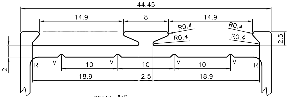
DETAIL "A" SCALE 3:1
