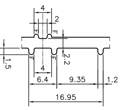
DETAIL OF "C" SCALE 3:1
