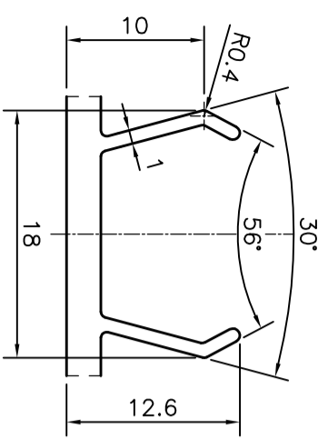
DETAIL OF "A" SCALE 2:1
