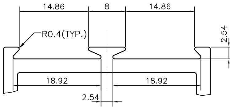
DETAIL AT "X"
