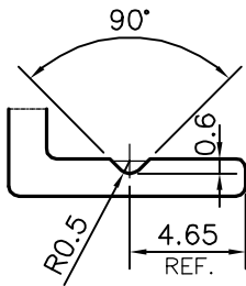
DETAIL OF "A" SCALE 3:1
