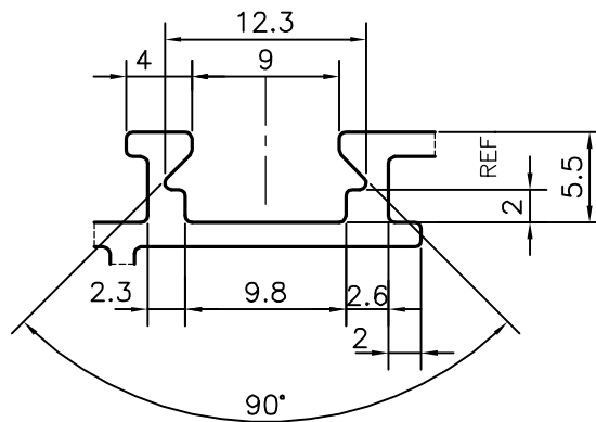
DETAIL OF "B" SCALE 2:1
