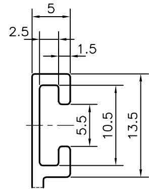
DETAIL OF "C" SCALE 2:1
