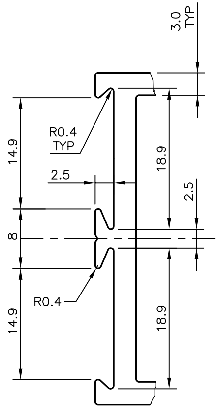
SCALE 2:1 DETAIL A
