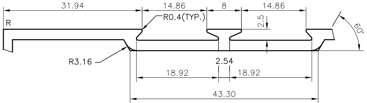
DETAILS - A (2:1)
