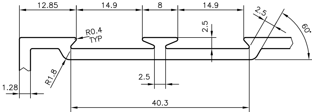
DETAILS - A (2:1)
