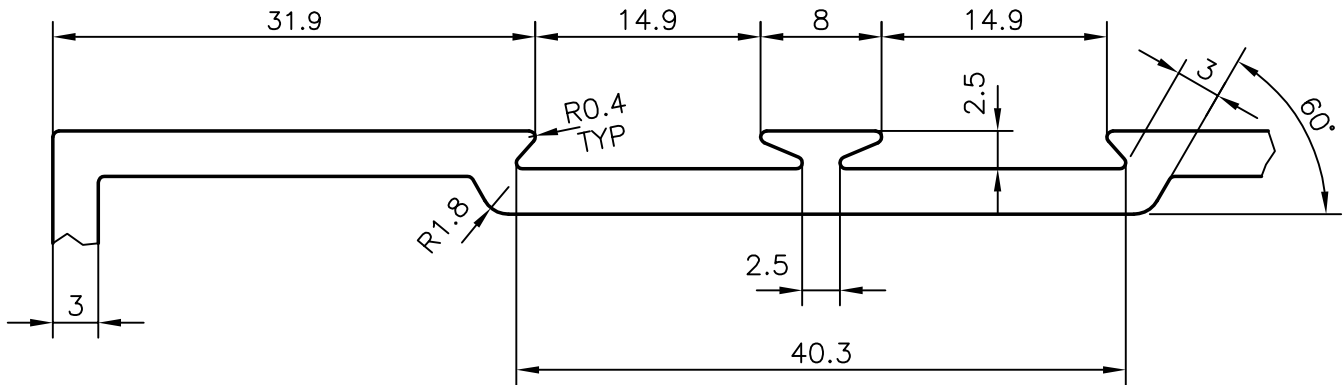
DETAILS - A (2:1)
