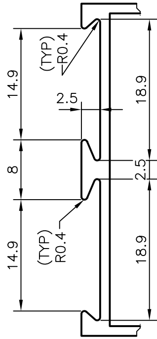
DETAIL AT 'A' (2:1)
