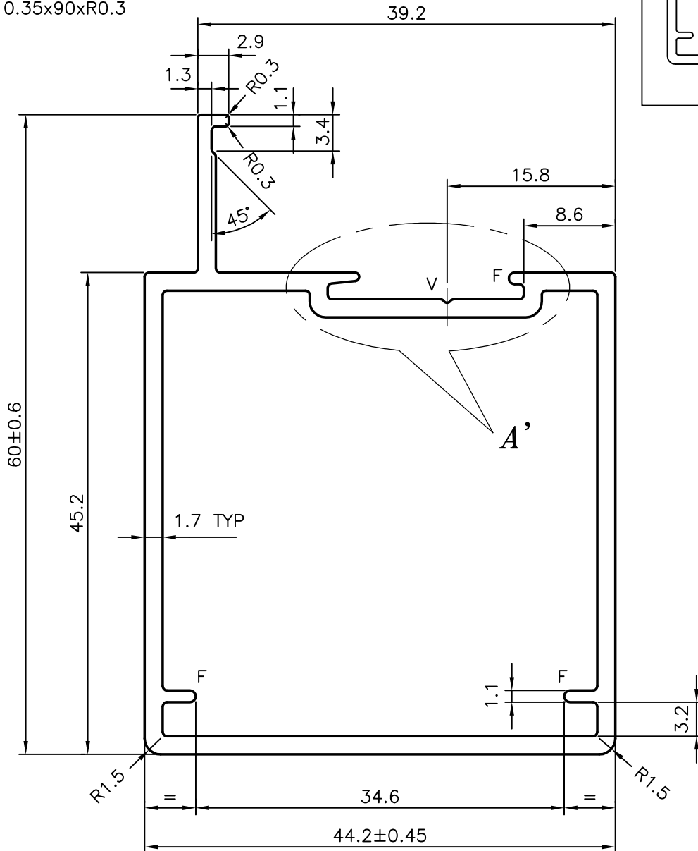
DETAIL-A
