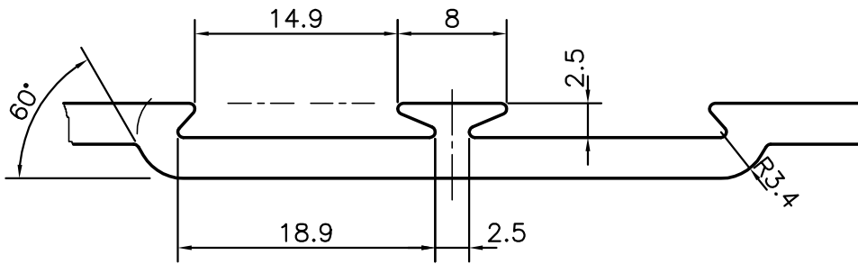
DETAIL OF 'A' SCALE 2:1
