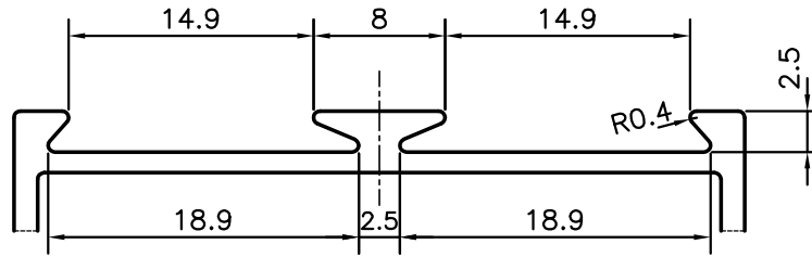
DETAIL OF "A" SCALE 2:1
