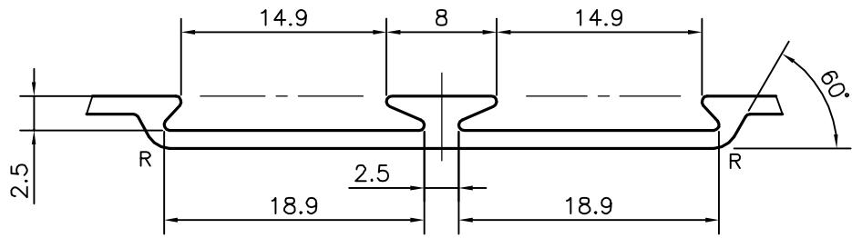
DETAILS OF "A" SCALE 2:1
