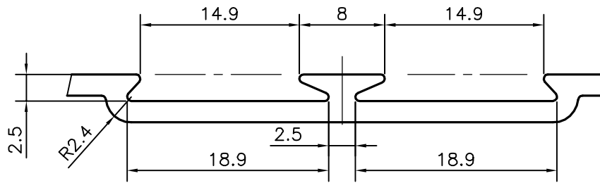
DETAILS OF "A" SCALE 2:1
