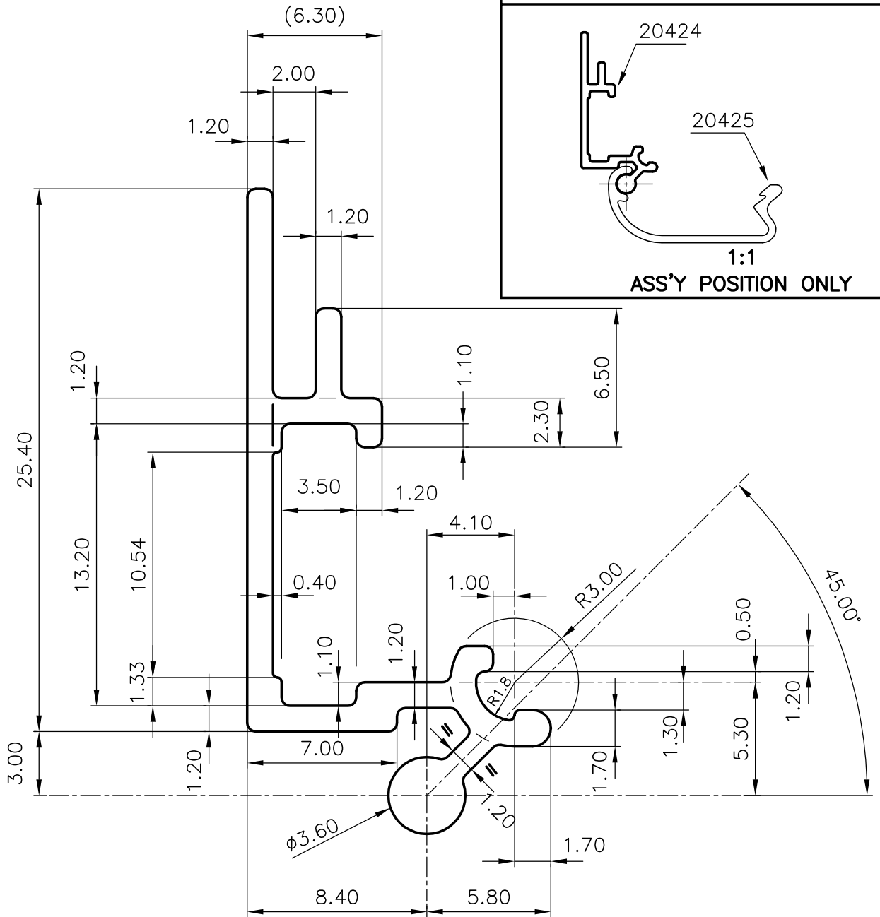
1:1 EXTRUDE MANUFACTURE SHAPE
