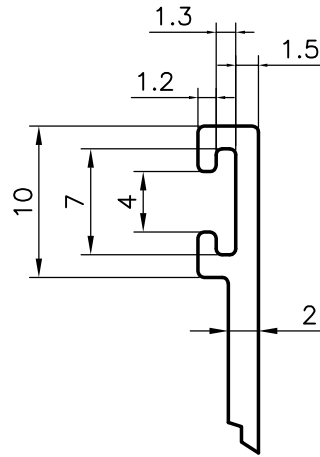
DETAL AT 'A'
