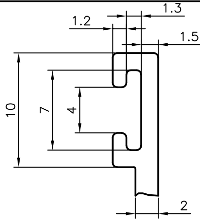
DETAIL AT 'A' SCALE 3:1
