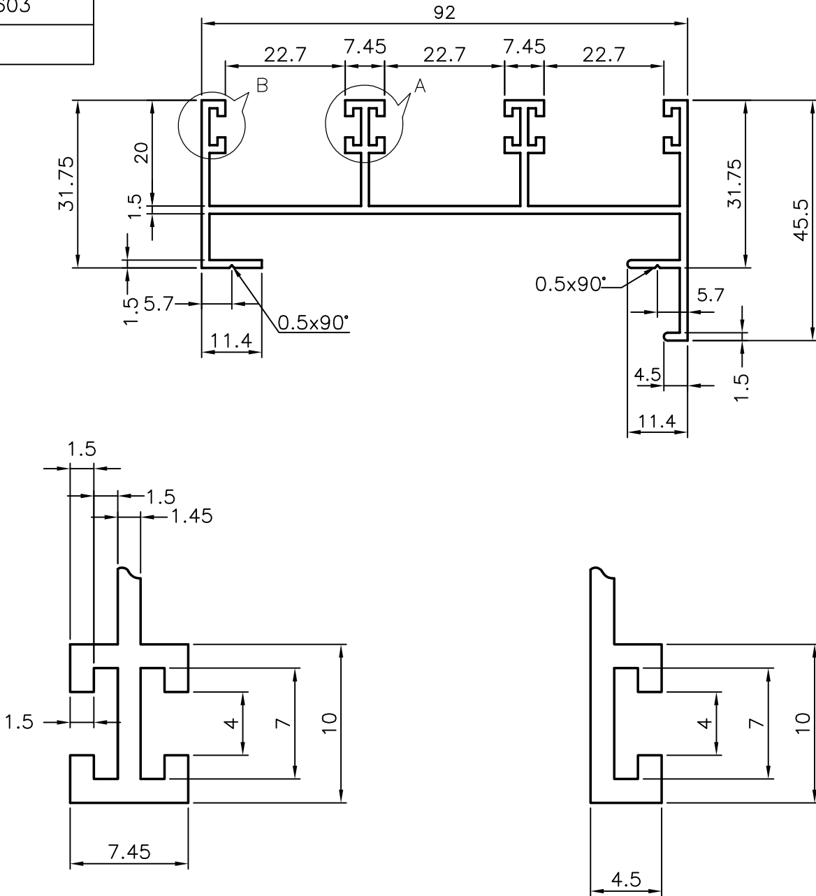
DETAIL AT 'A' SCALE 3:1
