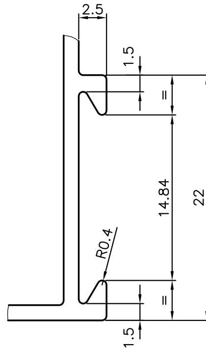
DETAIL OF "A" SCALE :- 3:1
