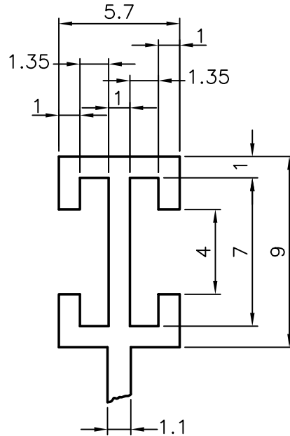
DETAIL AT-B
