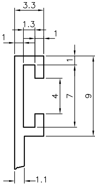
DETAIL AT- A
