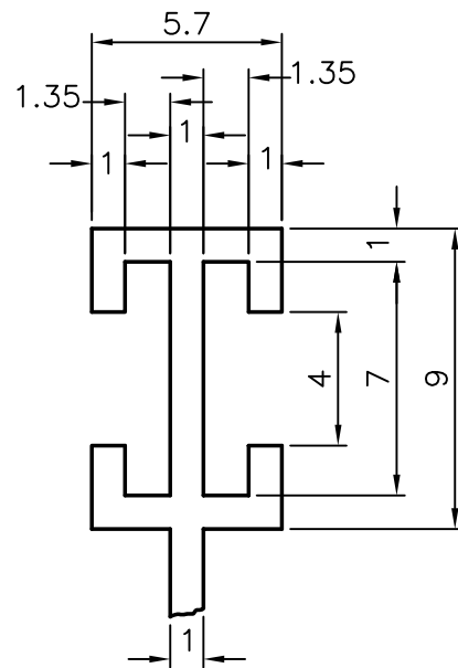
DETAIL - B
