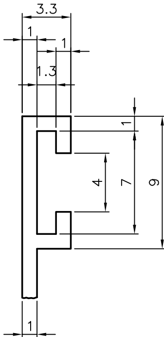
DETAIL - 'A'
