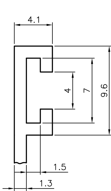
DETAIL-A
