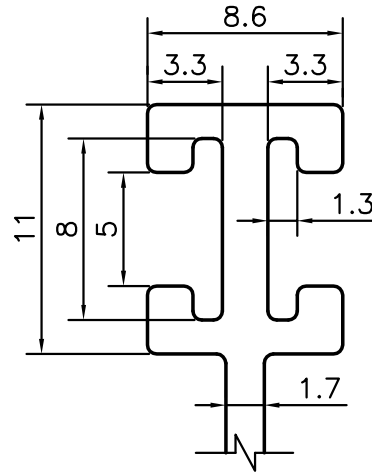
DETAIL OF "A" SCALE 3:1
