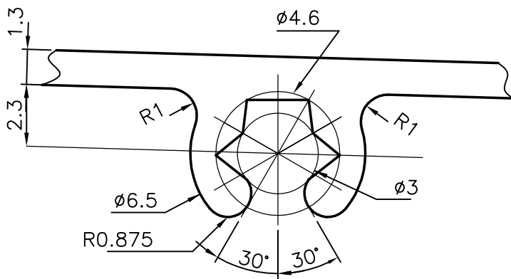
DETAIL OF 'A'
