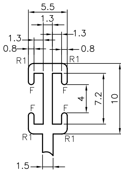
DETAIL AT 'B'
