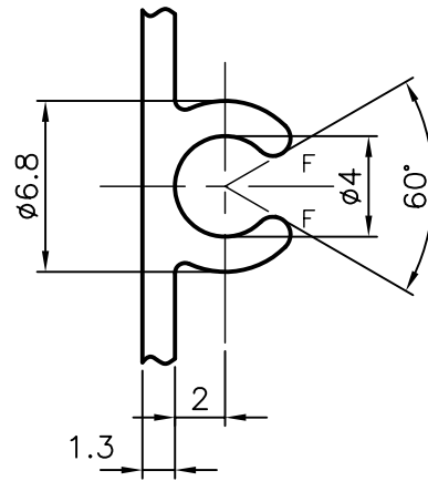
DETAIL AT 'A' (TYP.) SCALE 3:1
