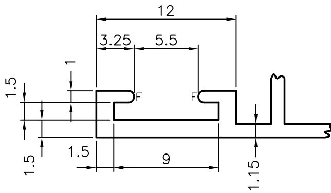
DETAIL 'A'
