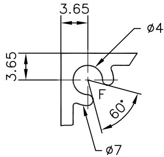
DETAIL AT "A"
