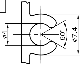
DETAIL AT 'A' (TYP)
