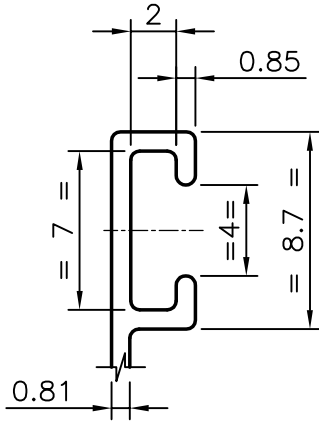
DETAIL OF "A" SCALE 3:1
