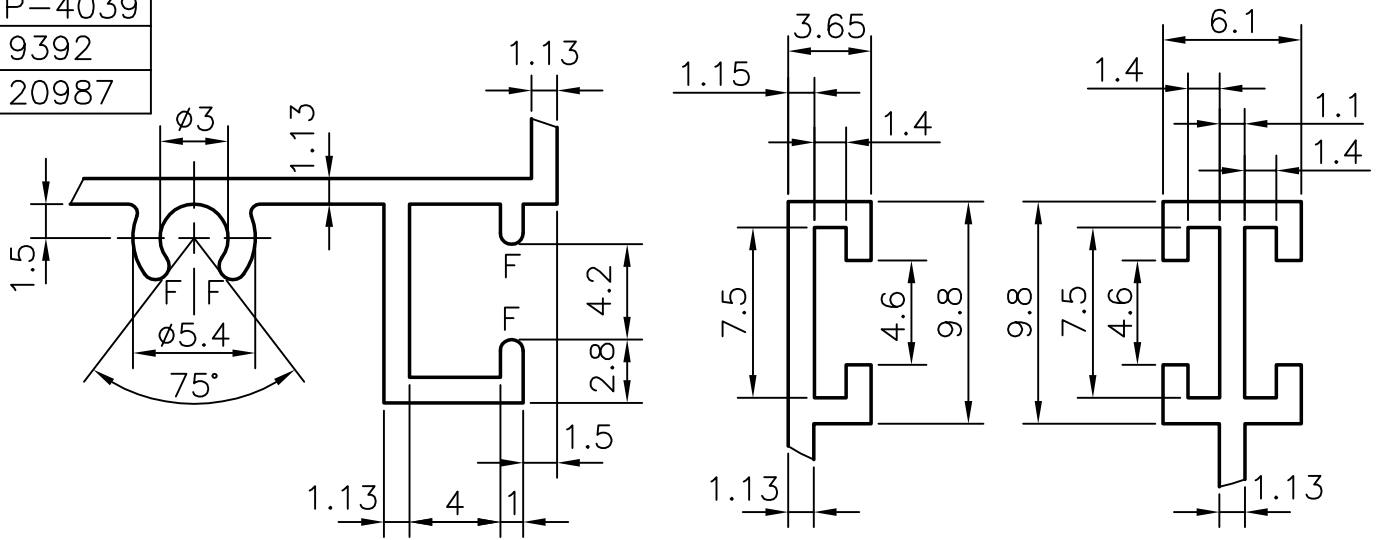
DETAIL 'C'
