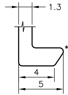
DETAIL AT 'A' (SCALE 4:1)
