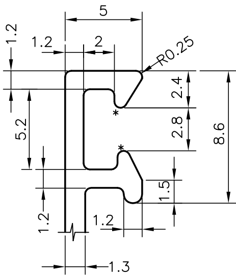
DETAIL AT 'B' (SCALE 4:1)
