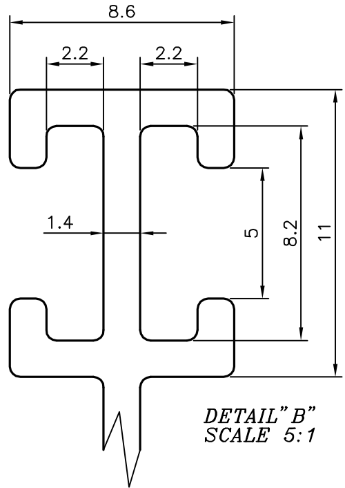
DETAIL "B"
