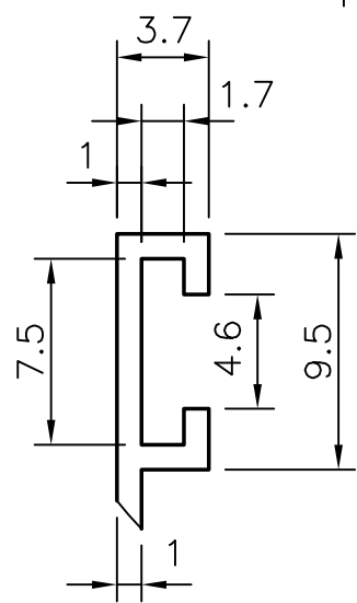
DETAIL 'A' (3:1)
