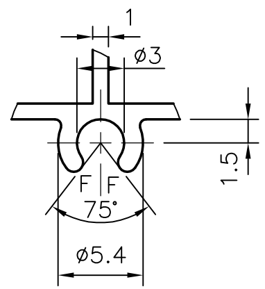
DETAIL 'C' (3:1)
