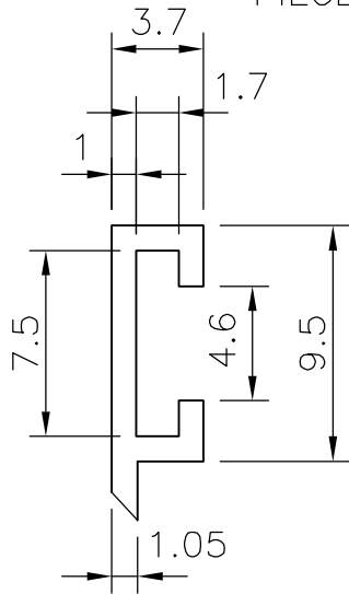
DETAIL 'A' (3:1)
