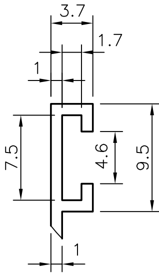
DETAIL 'A' (3:1)
