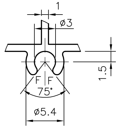
DETAIL 'C' (3:1)
