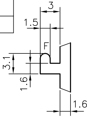
DETAIL 'C' (3:1)
