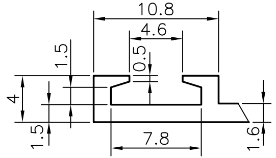
DETAIL 'A' (3:1)
