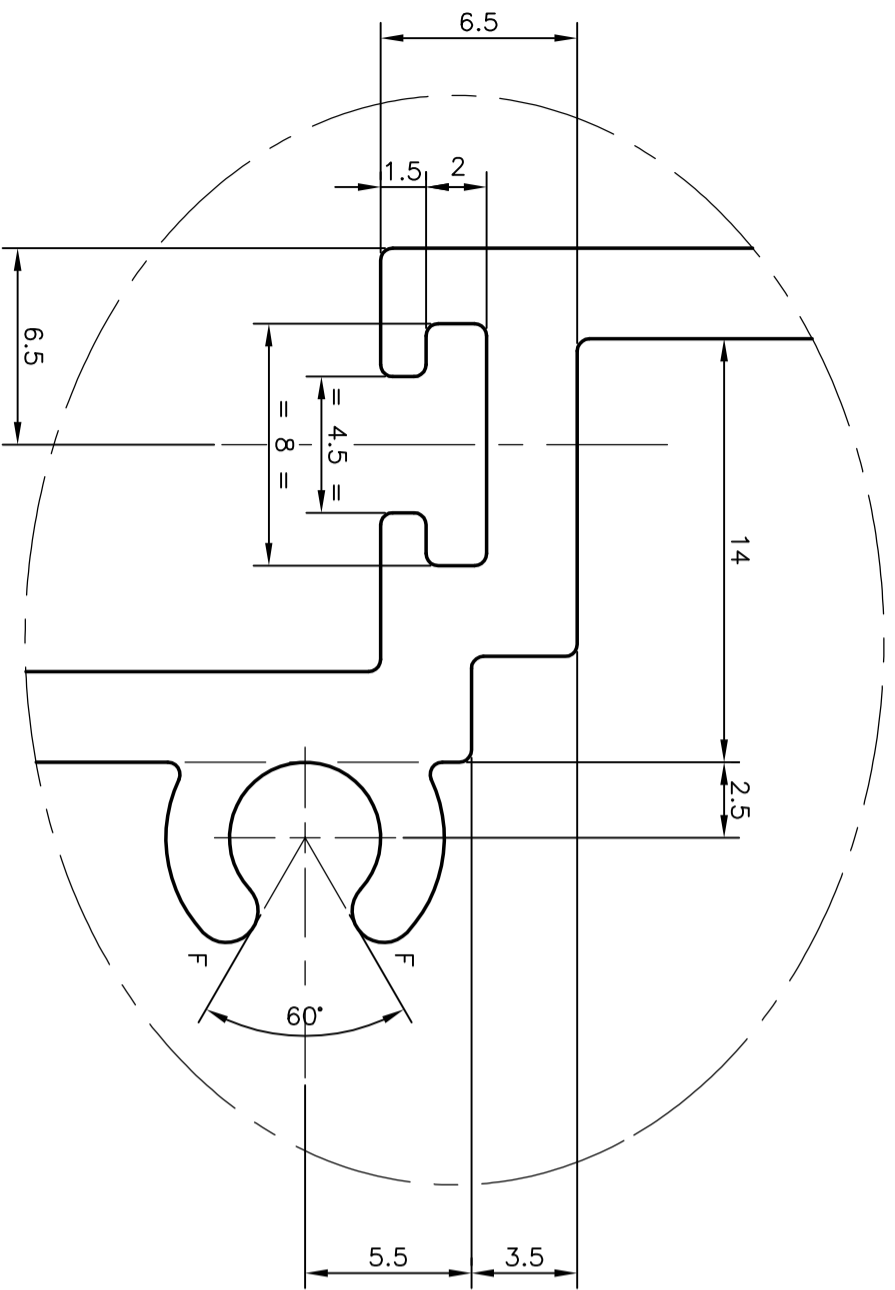
DETAIL-C SCALE:-4:1
