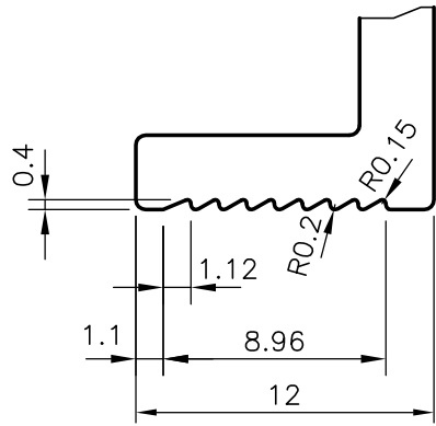
DETAIL AT-A
