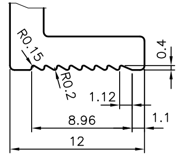
DETAIL AT-A
