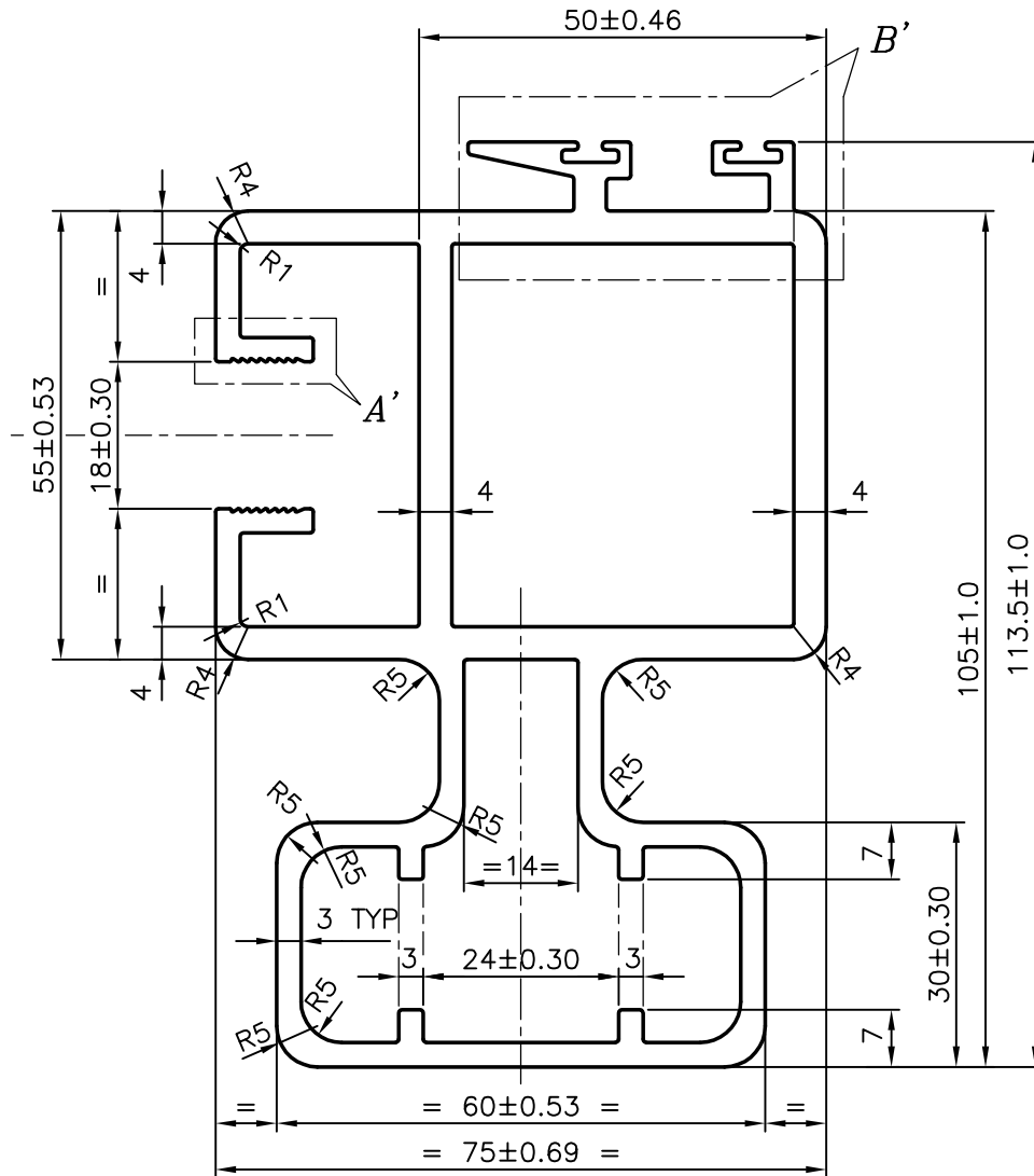
DETAIL AT-B
