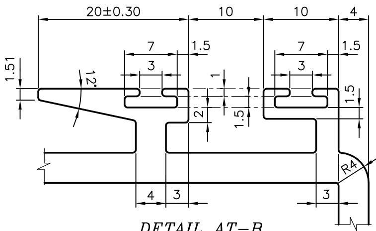
DETAIL AT-B
