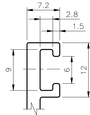
DETAIL OF "A" SCALE 2:1
