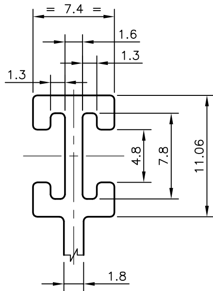
DETAIL OF "B" SCALE 3:1
