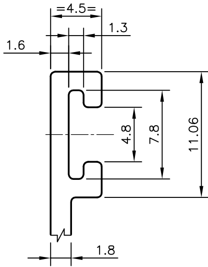
DETAIL OF "A" SCALE 3:1
