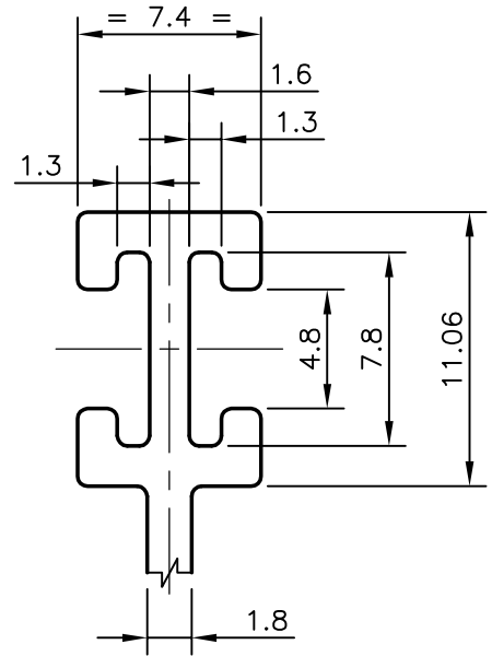
DETAIL OF "B" SCALE 3:1
