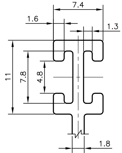
DETAIL OF "B" SCALE 3:1
