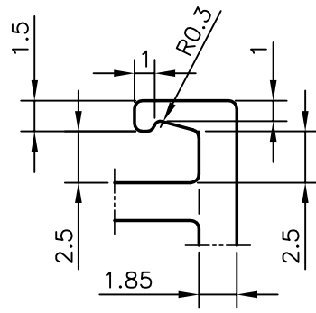
DETAIL OF "A" SCALE 3:1
