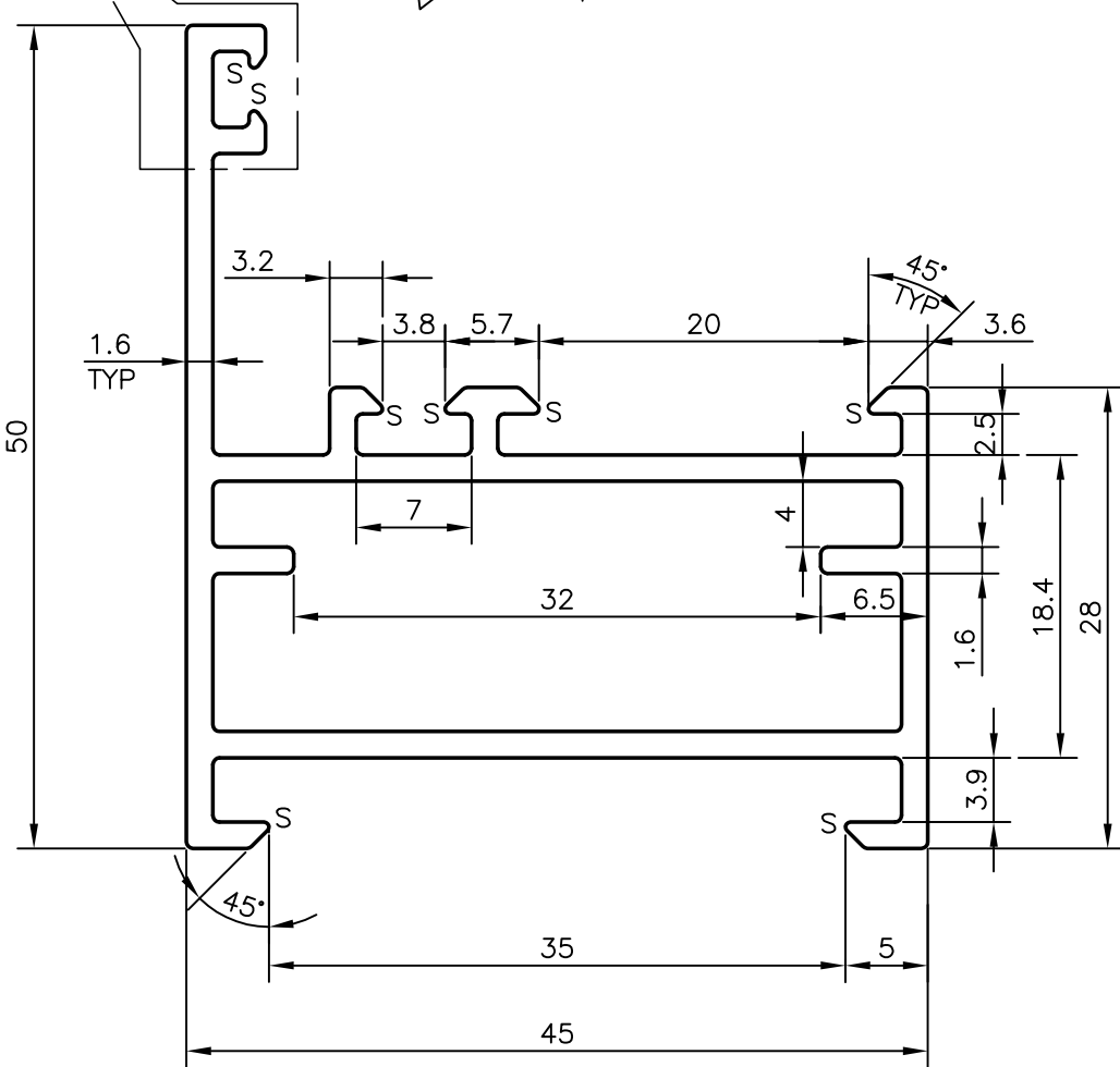
MATCHING SECTION SCALE 1:1
