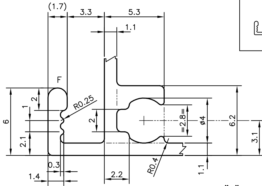
DETAIL OF "A" SCALE 5:1
